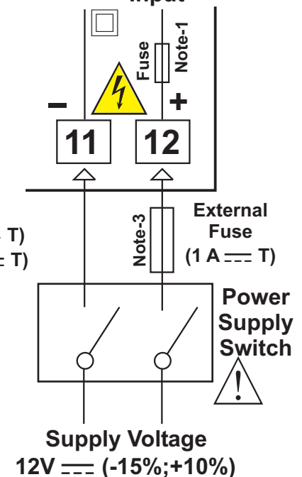
Connection of Low Voltage 12V=== Supply Voltage Input
