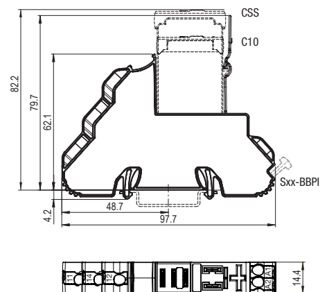
fig. 2. Dimension (mm)
