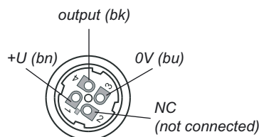
inside of the connector socket (var. "C")
