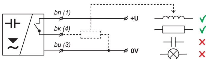
PNP type sensors connection
