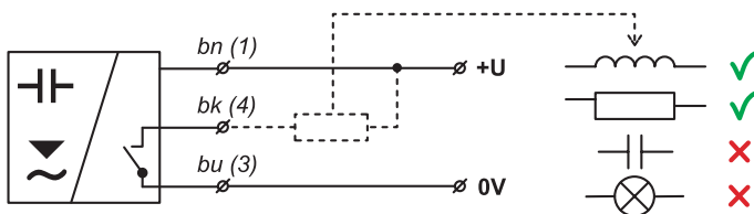
NPN type sensors connection
