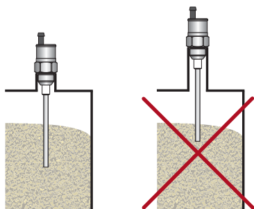
Fig. 12: Long fitting tubes in vertical mounting
