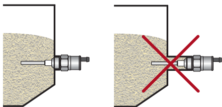
Fig. 2: Long fitting tubes in side wall mounting
