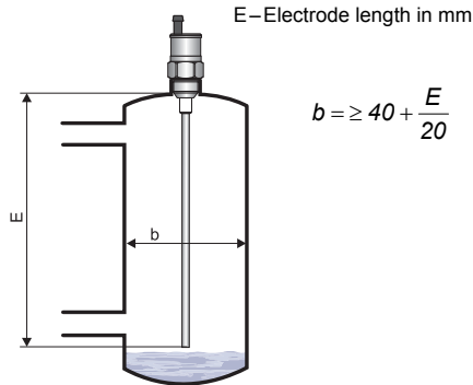
Fig. 8: Bypass measuring tube
