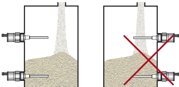
Fig. 3: Side wall mounting
