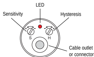
Fig. 17: Top view of level sensor
