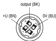
Fig. 16: Inside of the connector socket
