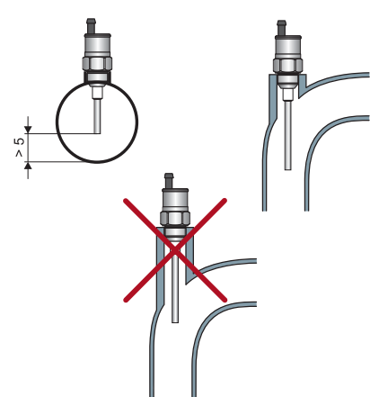
Fig. 10: Mounting in the pipe
