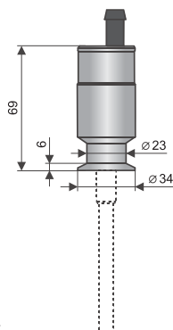
Tri-clamp process coupling
