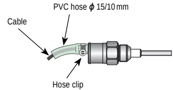
Fig. 9: Protective hose install
