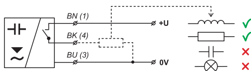
Fig. 14: PNP type sensors connection (version "N", "NT", "Xd")
