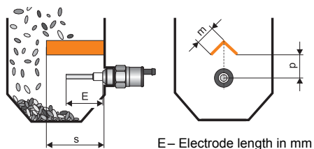
Fig. 4: Protective roof mounting
