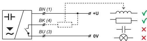
Fig. 13: NPN type sensors connection (version "N", "NT", "Xd")
