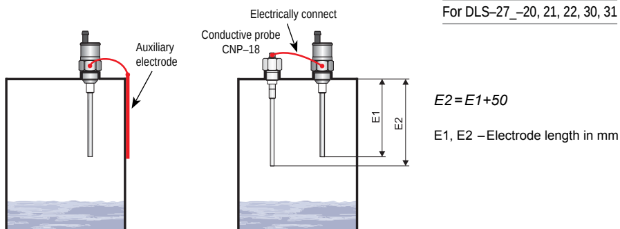
Fig. 6: Auxiliary electrode in non-conductive tanks
