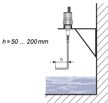
Fig. 7: Vertical installation for non-conductive fluids
