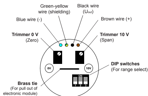
The top view on the internal electronic module for voltage output (var. -U )
