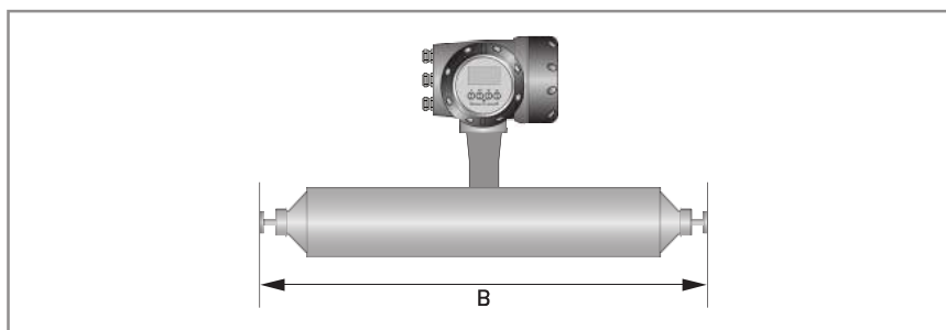
Dimension B: adapter versions (male thread)
