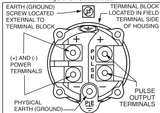
Figure 13. Terminal Block
