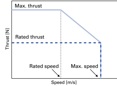
Thrust-Speed Characteristics
