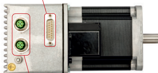
M12 EtherCAT IN / OUT connectors
