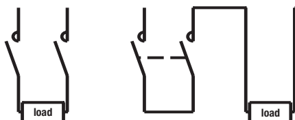
2 poles in series
