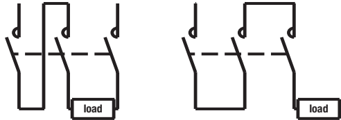
3 poles in series
