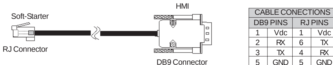
Figure 19.1 - Cable CAB-RS for HMI-SSW05-RS.
