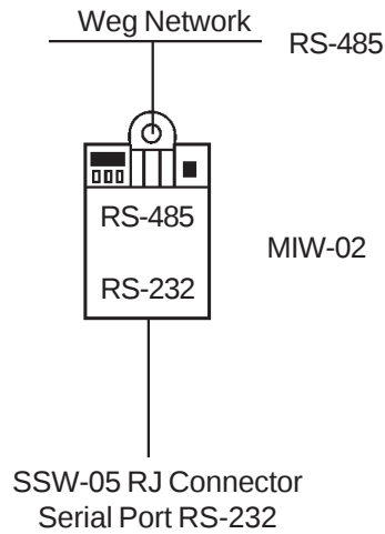
Figure 19.2 - Connection of the SSW-05 to a standard RS-485 communication network.
