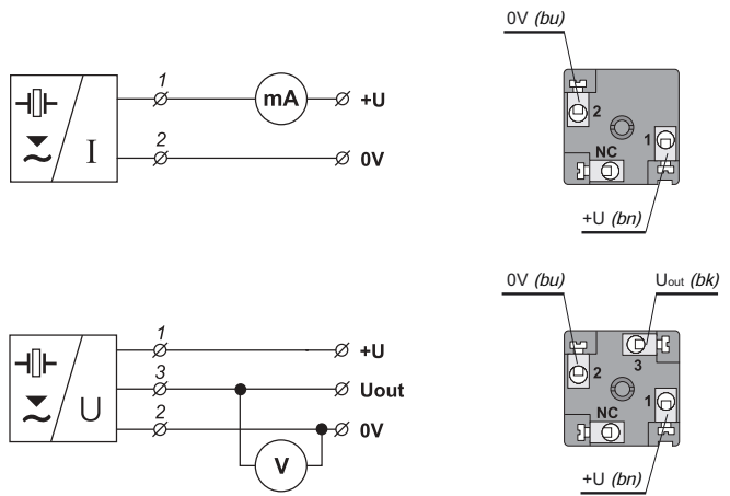
Connection scheme
