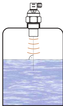
Recommended installation
