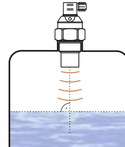
Fig. 1: Recommended installation in the tank
