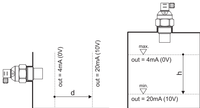
Fig. 18: Inverse mode (distance measurement)
