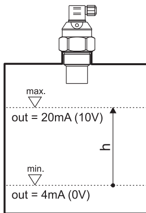
Fig. 17: Basic mode (measurement of level height)
