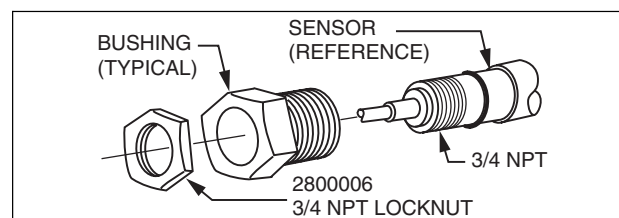
Figure 3. Typical Bushing Assembly
