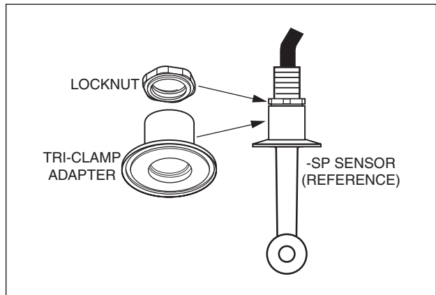
Figure 5. Tri-Clamp Mounting Kit
