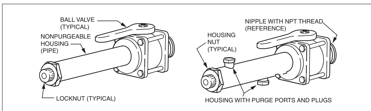
Figure 1. Typical Ball Valve Assemblies
