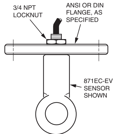
TYPICAL FLANGE MOUNTING CONFIGURATION
