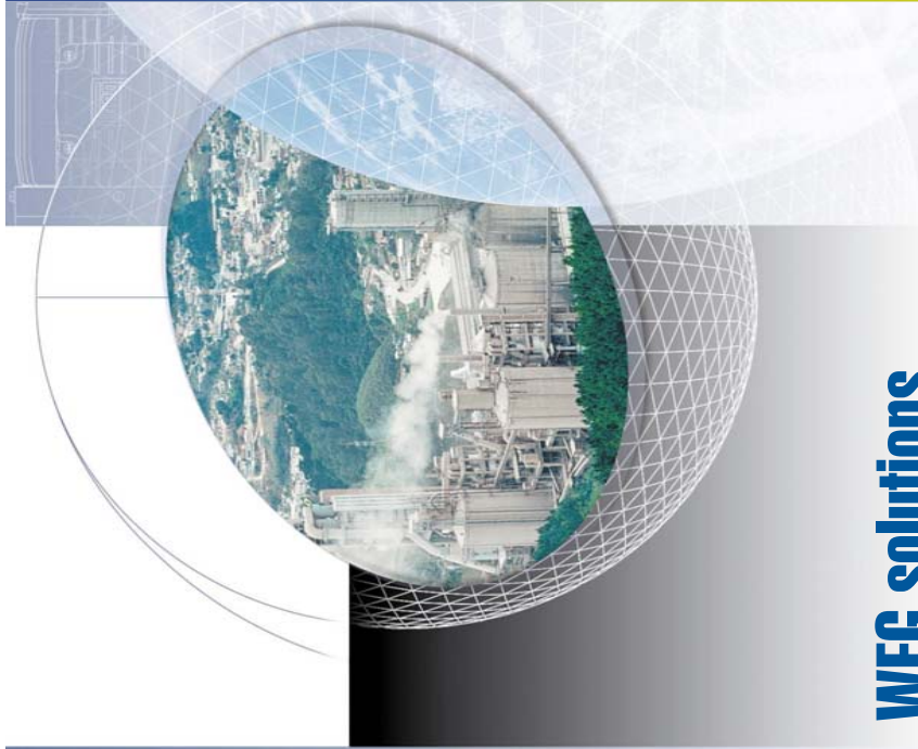
2 x 4200 kW, 6 pole, 6600 V, KA8000 frame motors Application: Mill
