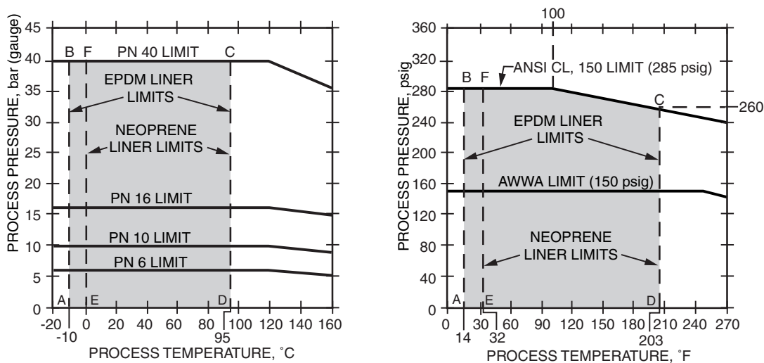
Figure 1. Flowtube Process Pressure-Temperature Limits with Various Liners, and ANSI/DIN Flanges
