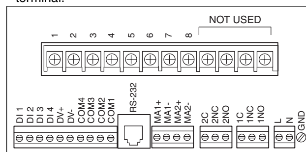
Figure 5. Wiring Terminal Configuration and Designation
