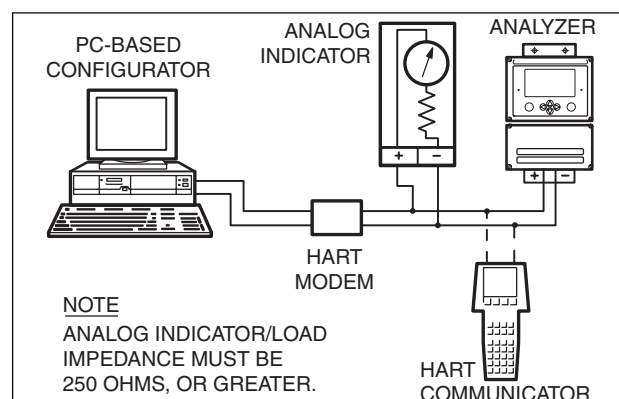
Figure 6. Point-to-Point Communications 4 to 20 mA Output with HART
